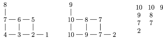
Figure 1. From left to right: A column-strict labelling \omega of P_\lambda with \lambda = (3, 2, 2, 1) , a (P_\lambda, \omega) -partition and the corresponding reverse SSYT.
