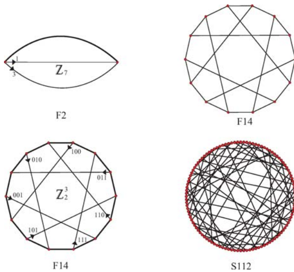
Fig. 8 Construction of S112 via a regular Z_7 -cover of F2 and a regular Z_2^3 -cover of F14
