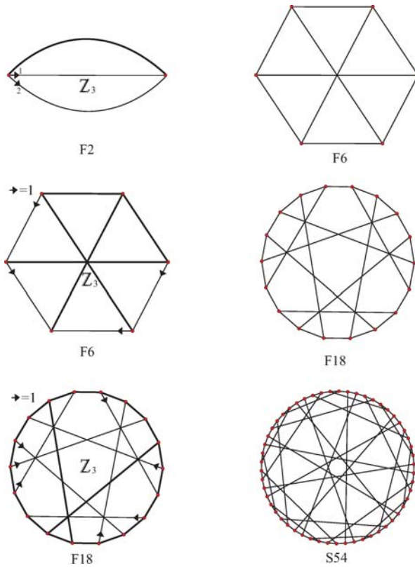
Fig. 7 A sequence of three regular Z_3 -covers leading to the Gray graph S54
