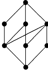
Figure 1. A non-Eulerian poset P with \Psi(P) \in \mathcal{F} .
