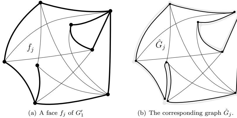
Figure 1: Illustrations for the proof of Proposition 3.
