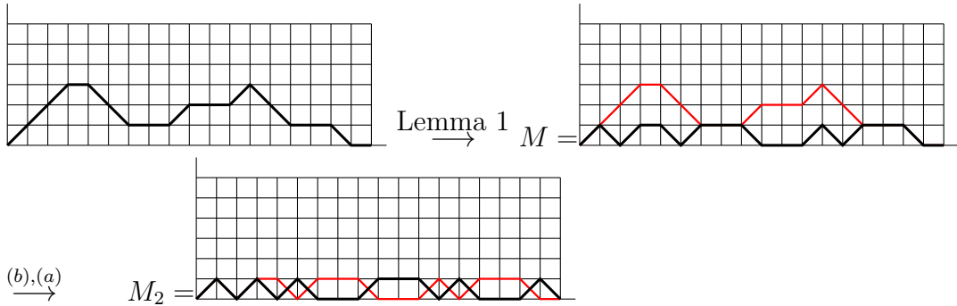
Figure 8: Illustration of the example in the proof of Lemma 15.
