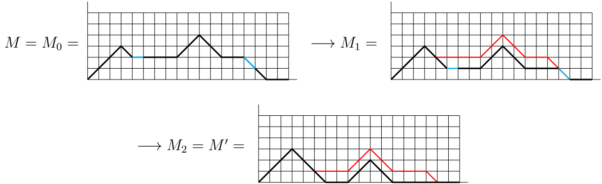
Figure 3: Illustration of the example described in the proof of Lemma 3.
