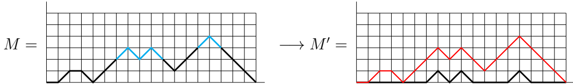
Figure 6: Illustration of the example in the proof of Lemma 9.
