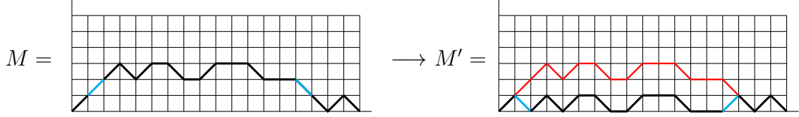
Figure 2: Illustration of the example described in the proof of Lemma 1.
