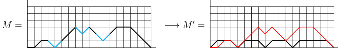
Figure 5: Illustration of the example in the proof of Lemma 9.
