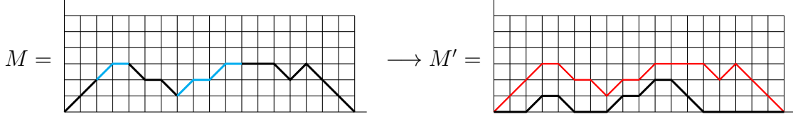
Figure 7: Illustration of the example in the proof of Lemma 11.
