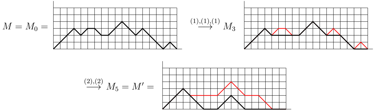
Figure 4: Illustration of the example described in the proof of Lemma 5.
