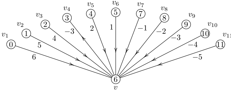
Figure 6: Illustrating the labeling g of the orientation D' of K_{1,11} in Proposition 3.3 for k = 3 and n = 12
