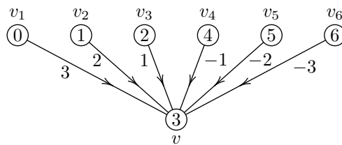
Figure 5: Illustrating the labeling f of the orientation D of K_{1,6} in Proposition 3.3 for k = 3 and n = 7
