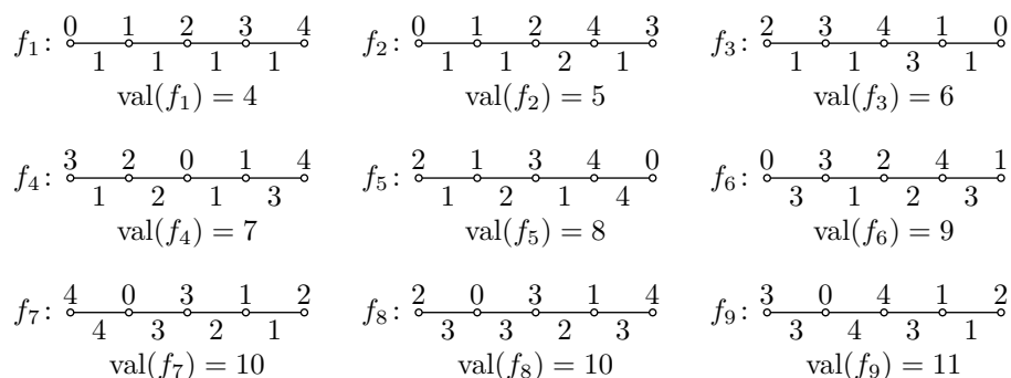
Figure 1: Some \gamma -labelings of P_5
