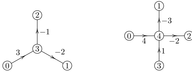
Figure 4: Illustrating \gamma -labelings of orientations of K_{1,3} and K_{1,4}
