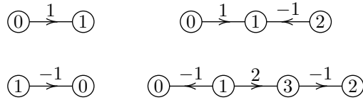
Figure 3: Illustrating \gamma -labelings of orientations of P_2 , P_3 , and P_4
