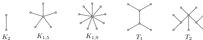
Figure 8: Trees that are not orientably balanced
