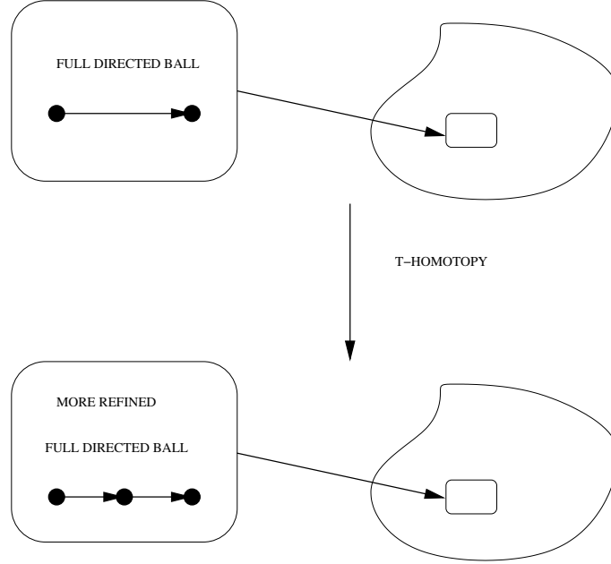
FIGURE 3. Replacement of a full directed ball by a more refined one
