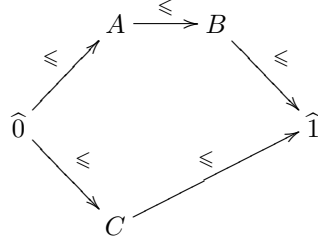
FIGURE 4. Example of finite bounded poset
