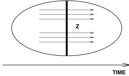
FIGURE 1. Symbolic representation of \text{Glob}(Z) for some topological space Z
