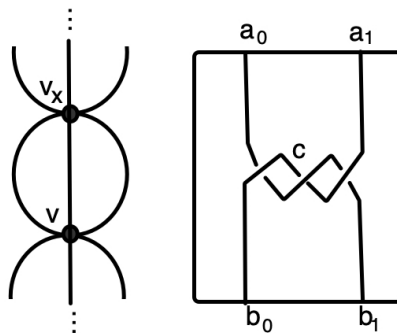
FIGURE 9. 1-periodic graph G and associated tangle diagram D_0
