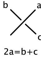
FIGURE 5. Fox coloring relation
