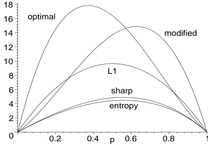
FIG 1. Graph of the entropy as a function of p .
