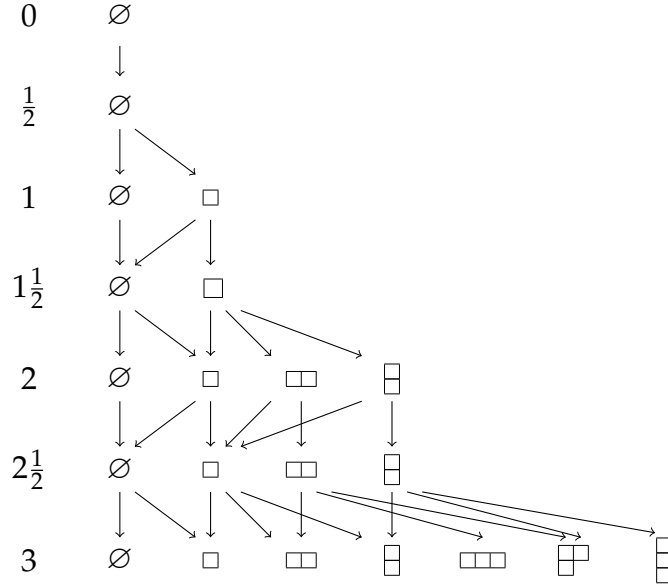
Figure 1: The first three layers of the branching graph \mathcal{Y}
