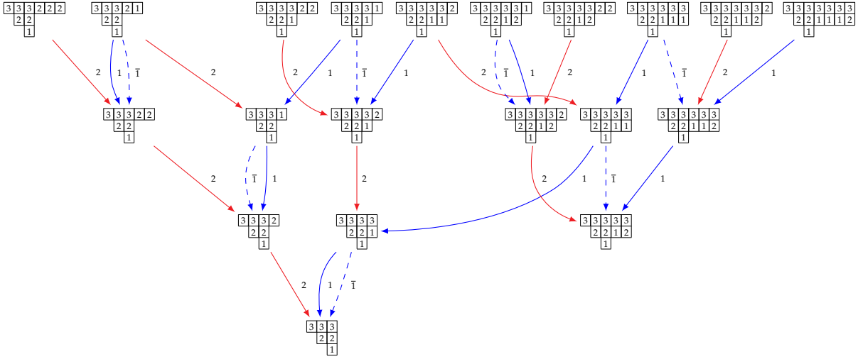
Figure 3.1: A bottom portion of the q(3) -crystal \text{SDT}(-\infty) containing the lowest weight element L^{-\infty} created using SAGEMATH [4].
