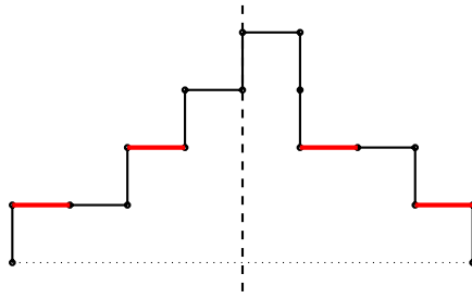
Figure 4: A unimodal bargraph B with \text{ds}(B) = 2 , e(B) = 8 and n(B) = 4 , corresponding to the composition (1, 1, 2, 3, 4, 2, 2, 1) .
