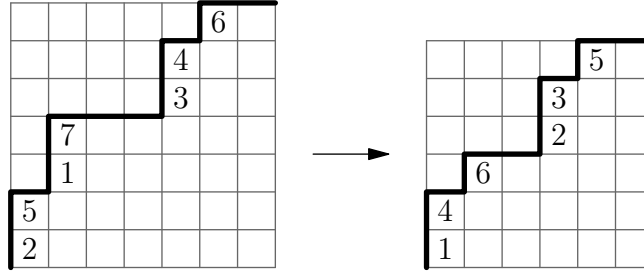
Figure 2: An illustration of the map P \mapsto P' described in the proof of Theorem 1.1 .
