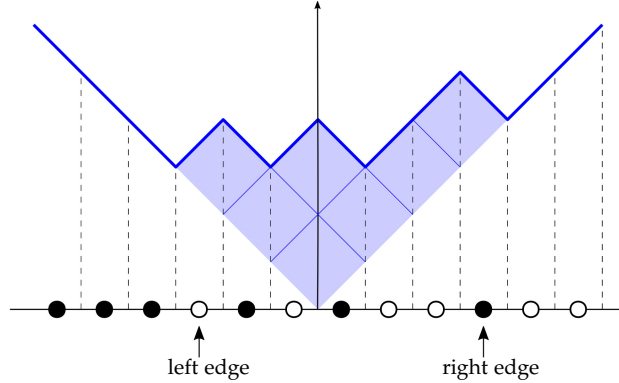
Figure 1: The profile (thick blue line) and the set S(\lambda) = \{\frac{7}{2}, \frac{1}{2}, -\frac{3}{2}, -\frac{7}{2}, -\frac{9}{2}, \dots\} (black dots, corresponding to the -1 slopes in the profile) for the partition \lambda = (4, 2, 1) .
