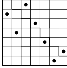
Figure 1: The permutation 3142576 is 321-avoiding: in the upper triangle, as well as in the lower triangle, the dots come in a strictly falling spread.
