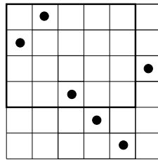
Figure 2: An extendably 321-avoiding 4 \times 5 -matrix with three dots (indicated with bold border), extended to a 321-avoiding permutation matrix.
