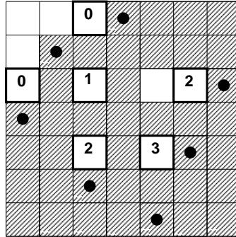
Figure 4: Diagram and ranked essential set of the permutation 4271635.
