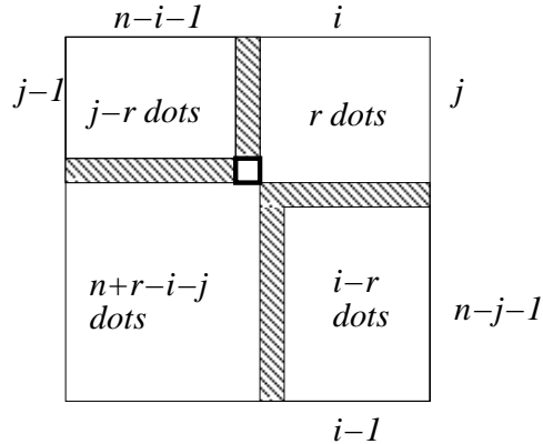
Figure 5: A 321-avoiding permutation with a northeast-rank r white corner at (i, j)^{\text{ne}} .
