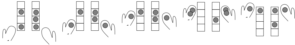
Figure 3: The game played from a bad situation. The left squares are \{\mathbf{r}_1, \mathbf{r}_2, \mathbf{r}_3, \mathbf{r}_4\} , the right squares are \{\mathbf{k}_2, \mathbf{k}_3, \mathbf{k}_4, \mathbf{k}_5\} .
