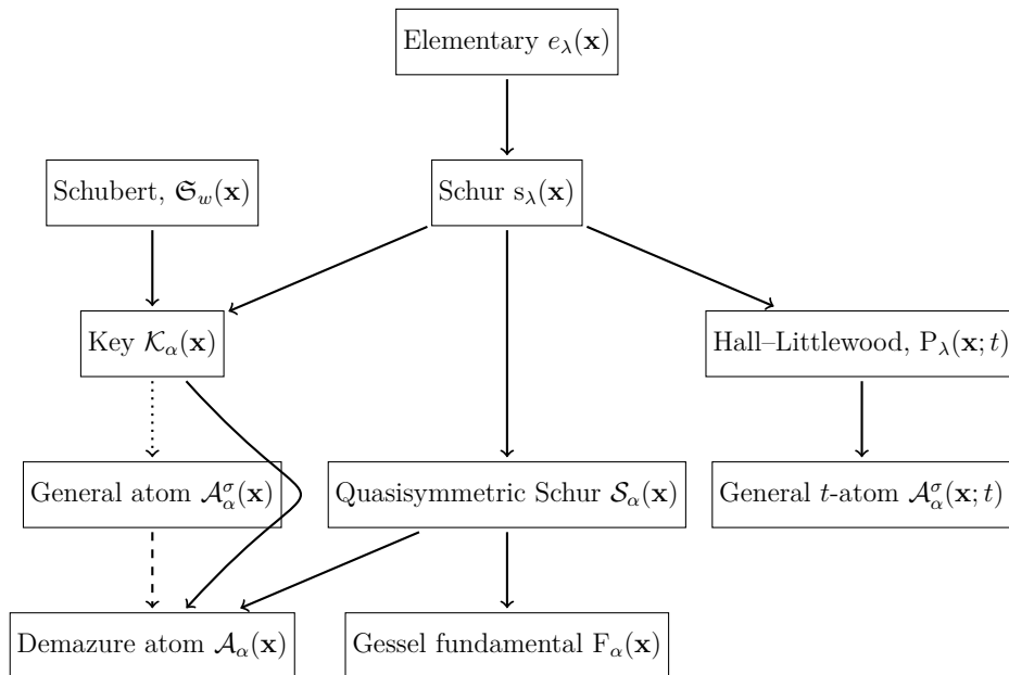
FIGURE 1. This graph shows various families of polynomials. The arrows indicate the relation expands positively in which means that the coefficients are polynomials with non-negative coefficients. A proof of the dashed edge can be found in [Pun16] and a generalization of the dotted edge is given in [AS19].
