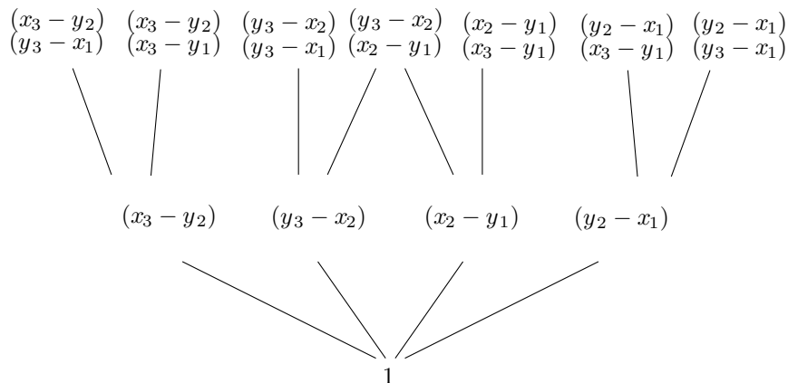
FIGURE 5. The polynomials associated to the quadrangulations of Figure 3
