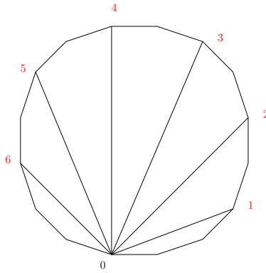
FIGURE 2. The fan Q_0 for m = 2 and n = 7
