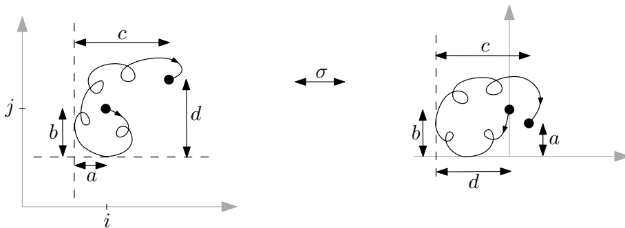
FIGURE 12. The bijection of Proposition 7.2 (derived from \sigma ) between \mathcal{Q}^{(i,j)} and \bigcup_{0 \leq a \leq i} \bigcup_{0 \leq b \leq j} \mathcal{H}^{b \rightarrow a} .
