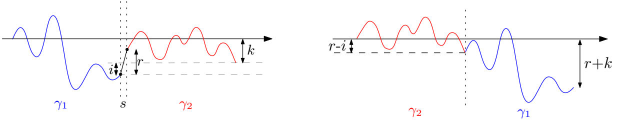
FIGURE 14. The bijection between \mathcal{N}_{k,r,i} (for any fixed i \leq r ) and \mathcal{W}_{k+r} .
