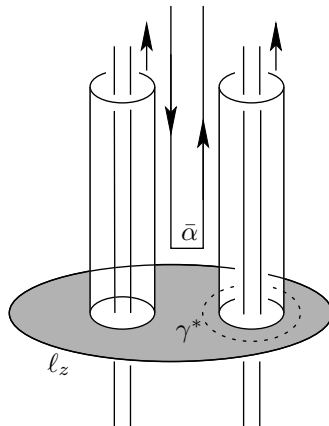
Figure 4: l_z = [\gamma^*, \bar{\alpha}]
