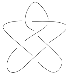
Figure 1: The knot 6_2
