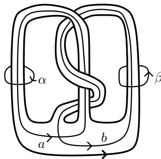
Figure 7.3: Seifert surface for 6_1
