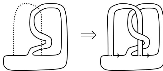
Figure 7.2: A ribbon disk for 6_1
