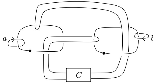
Figure 2.3: Handle decomposition of N_D , with generators a, b for \pi_1(N_D) .
