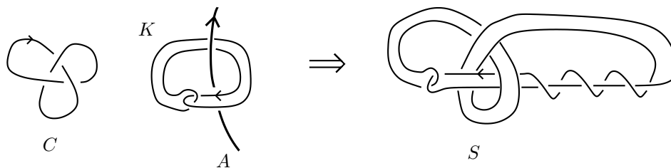
Figure 6.1: Satellite construction with C the trefoil, K the unknot
