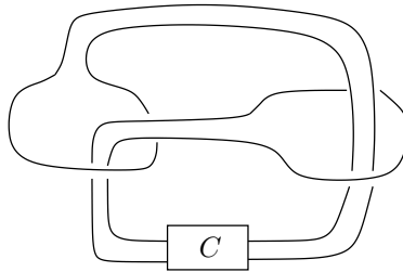
Figure 1.1: A family of ribbon knots
