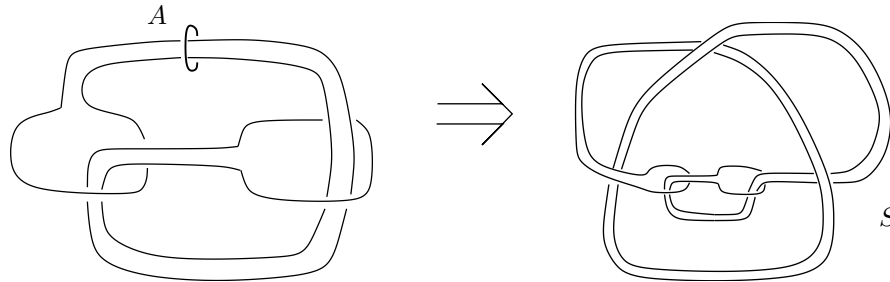
Figure 7.6: Ribbon knot with choice of A and the satellite knot S(6_1, \text{trefoil}, A)
