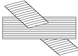
Figure 1.2: Local singularity of a ribbon
