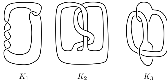
Figure 7.1: Three projections of the knot 6_1
