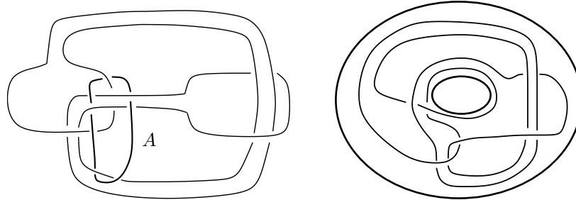
Figure 1.5: The knot 6_1 in the solid torus S^3 \setminus A
