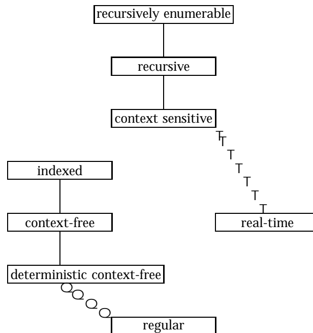
Figure 2: Inclusions between formal language classes
