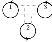
Figure 7: The only diagram contributing to F_3^{(2)}
