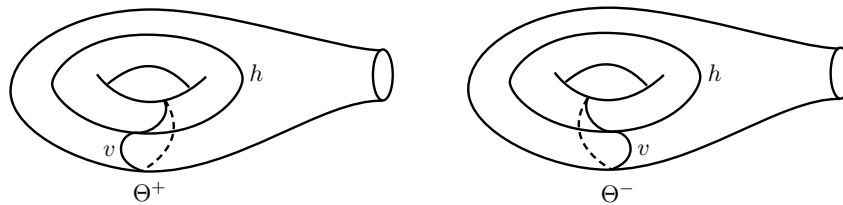
Figure 1: The train tracks \Theta^+ and \Theta^- on the once-punctured torus T
