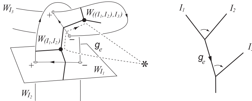
Figure 4: A Whitney disk W_{((I_1, I_2), I_3)} and its associated tree t(W_{((I_1, I_2), I_3)}) shown (left) as a subset of the Whitney tower and (right) as an abstract rooted tree. The boundaries of the Whitney disks are oriented according to our bracket-orientation conventions using the indicated signs of the intersection points. The dashed path indicates a sheet-changing loop (based at the basepoint of the ambient 4-manifold X ) which determines the element g_e \in \pi_1 X decorating the corresponding oriented edge as described in 3.5.
