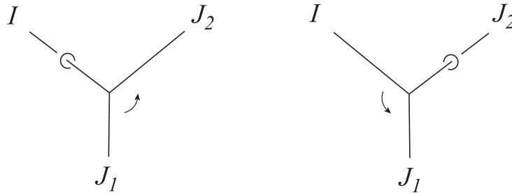
Figure 9: A local picture of the tree associated to the split subtower \mathcal{W} before (left) and \mathcal{W}' after (right) the Whitney move in the proof of Lemma 14 illustrated in Figure 10 and Figure 11.
