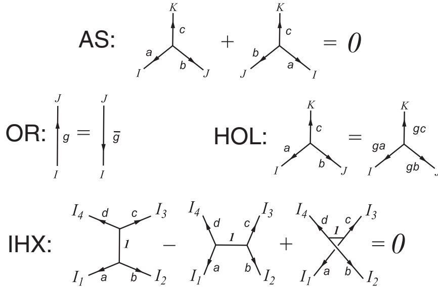
Figure 7: The AS, OR, HOL and IHX relations in \mathcal{T}_n(\pi, m) for a, b, c, d, 1 and g in \pi with \bar{g} = g^{-1} . All trivalent orientations are induced from a fixed orientation of the plane.
