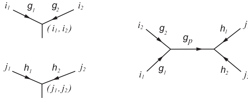
Figure 6: A pair of decorated rooted trees t(I) and t(J) corresponding to order-1 Whitney disks W_I and W_J with I = (i_1, i_2) and J = (j_1, j_2) (left), and the inner product t_p = t(W_I) \cdot_{g_p} t(W_J) = t(I) \cdot_{g_p} t(J) associated to an order-2 intersection point p \in W_I \cap W_J (right).
