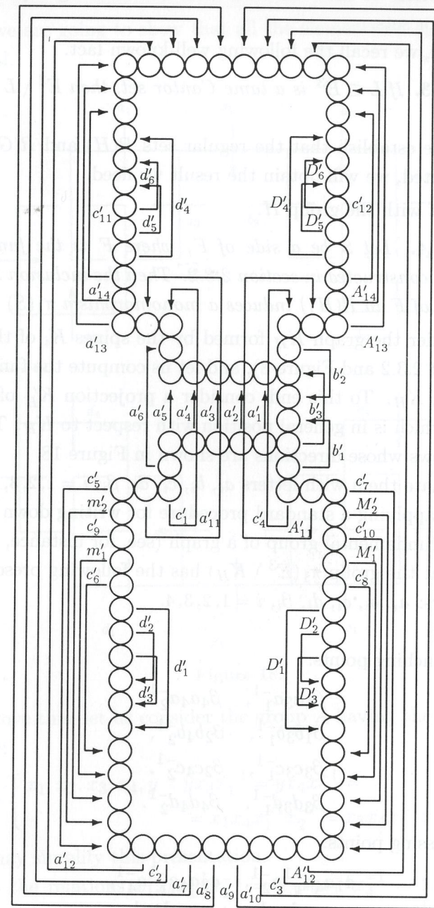
Figure 17: Fundamental domain and generators of G .
