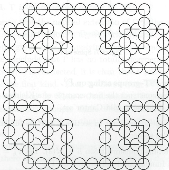
Figure 9: Fundamental domain for H .
