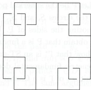
Figure 8: Link of spines.
