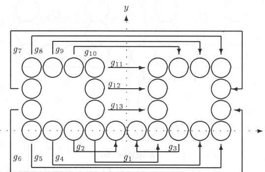
Figure 5: Fundamental domain of \Gamma .
