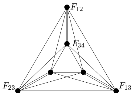
FIGURE 2. The 6B configuration
