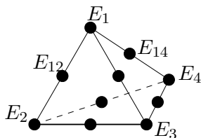
FIGURE 1. The 10A configuration.
