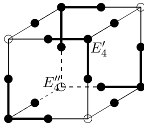
FIGURE 3. The quartic surface with four D_4 singularities.
