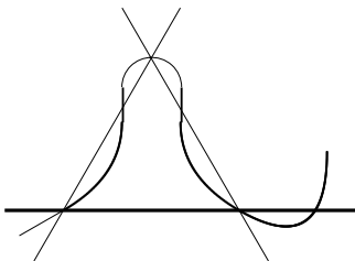
FIGURE 4. The branch sextic B
