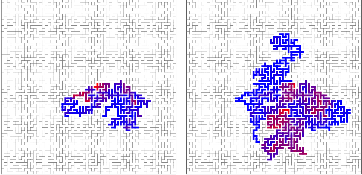
Figure 1: The range of a realisation of the simple random walk on uniform spanning tree on a 60 \times 60 box (with wired boundary conditions), shown after 5,000 and 50,000 steps. From most to least crossed edges, colours blend from red to blue.
