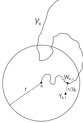
Figure 2: A sample of A_1(x, r, k) in Lemma 2.4.
