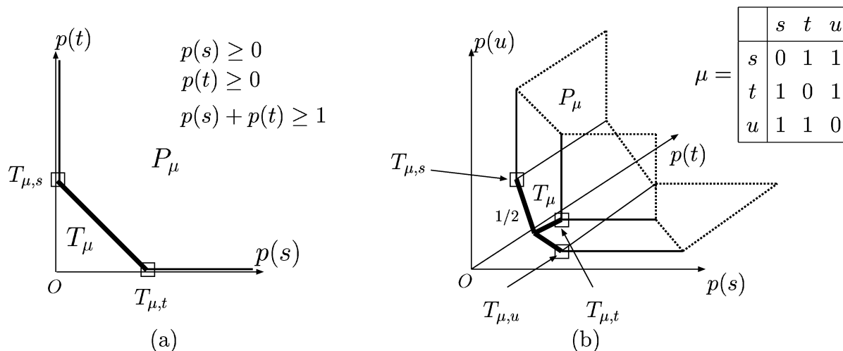
Figure 1. (a) T_\mu of a 2-point distance and (b) T_\mu of all-one 3-point distance
