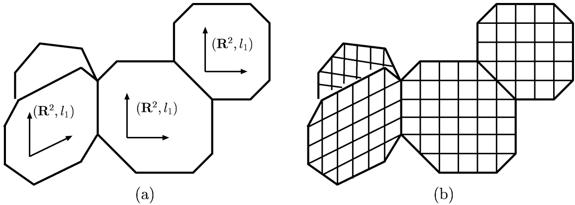
Figure 4. (a) gluing 2-faces and (b) an l_1 -grid
