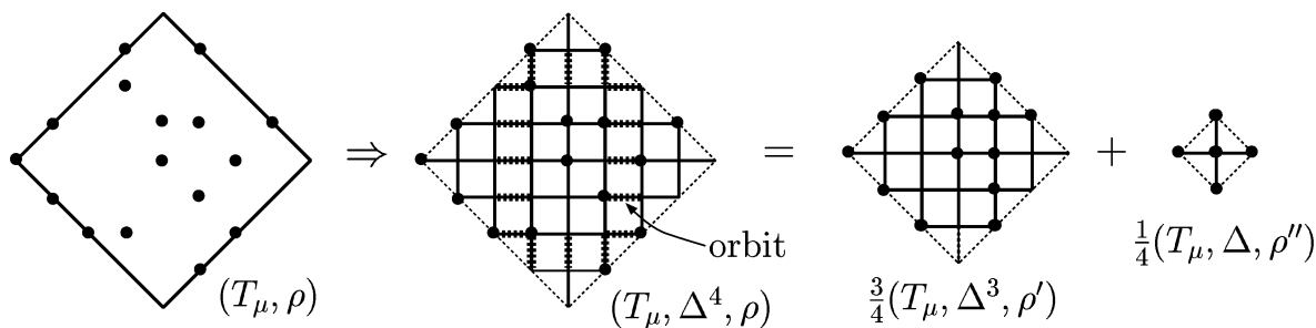
Figure 3. Subdividing and decomposing T_\mu
