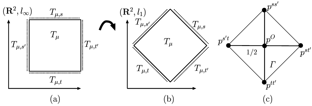
Figure 2. Two-commodity tight span
