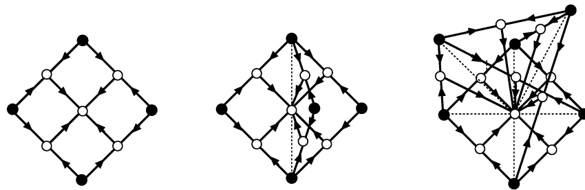
Figure 9. Subdividing and orienting folders
