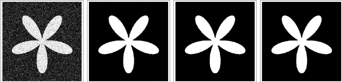
Figure 4. Example 3, EHM scheme: initial noisy image with 20 percent salt & pepper noise added (left), filtering results after 1 (middle) and 3 (right) and 10 time steps (extreme right).
