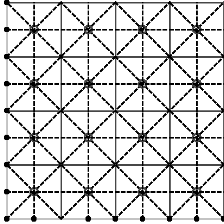
Figure 1. The co-volumes (solid gray lines), the triangulation for the co-volume method (dashed lines), and the degree of freedom (DF) nodes (round points), the part of boundary \partial\Omega (gray lines on the left and on the bottom of the figure) and the points where Dirichlet boundary condition is prescribed (black full points).
