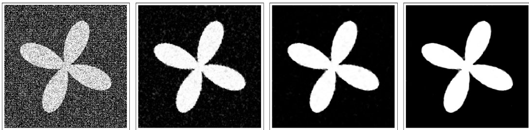
Figure 7. Example 4, CVS scheme: initial noisy image with 50 percent salt & pepper noise added (extreme left), filtering result after 1 (middle left), 3 (middle right) and 10 (extreme right) time steps.
