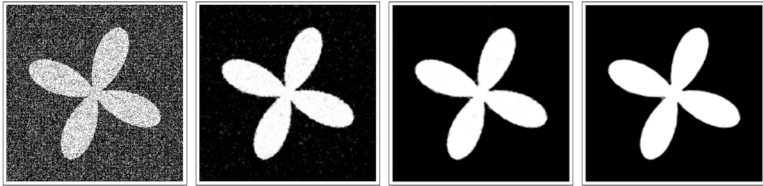
Figure 6. Example 4, EHM scheme: initial noisy image with 50 percent salt & pepper noise added (extreme left), filtering result after 1 (middle left), 3 (middle right) and 10 (extreme right) time steps.
