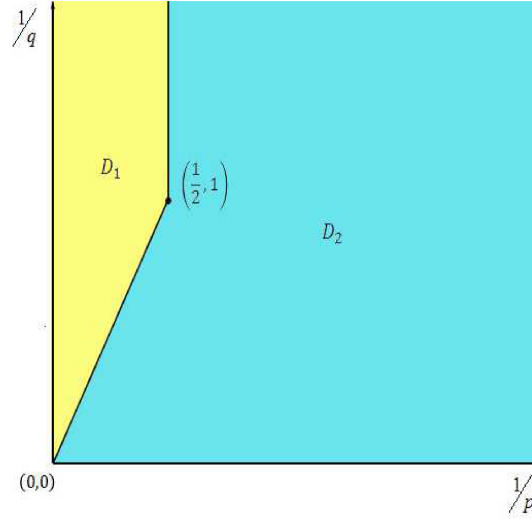
Figure 2. Distribution of s_0
