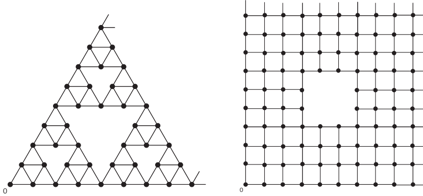
Fig 1: 2-dimensional Sierpinski gasket graph and carpet graph
