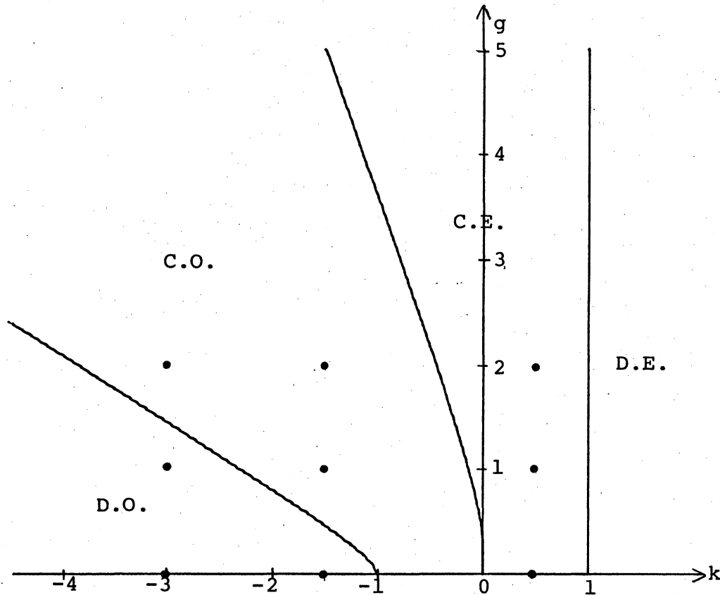
Stability Region
