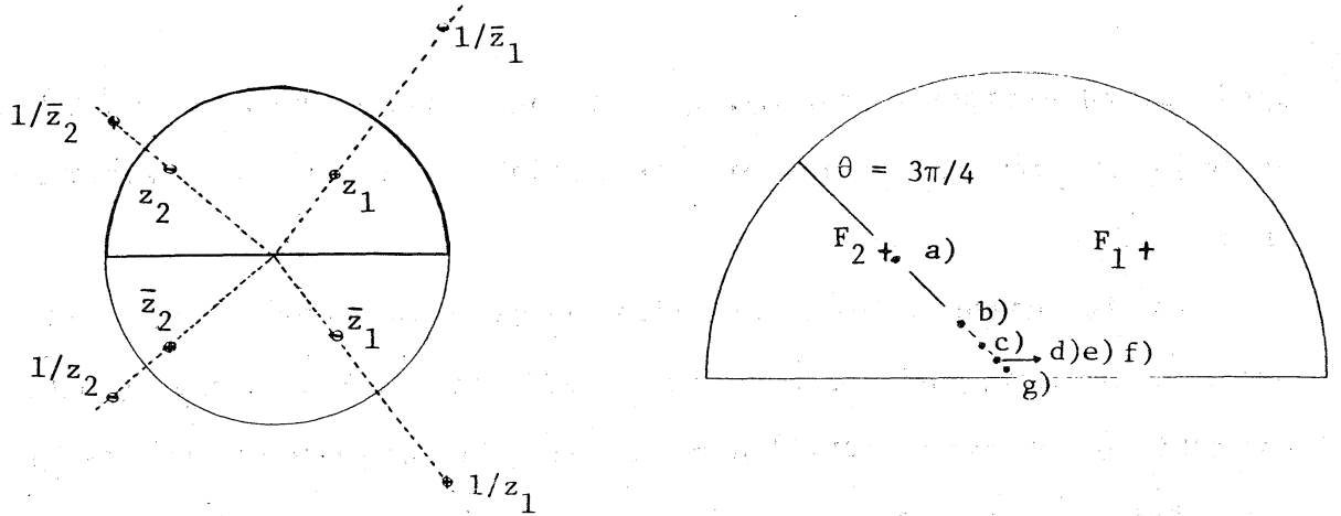
Fig. 1; The configuration of vortices Fig. 2; The change of initial conditi
