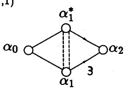
G_2^{(3,1)}
