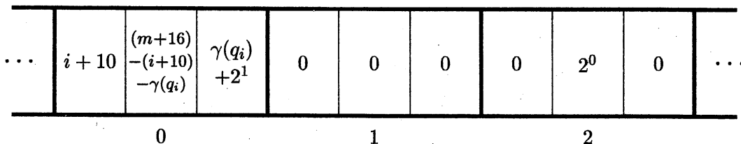
Figure 3: The configuration \varphi(q_i, 2, 0) such that q_i \in \text{Inc}_1 .
