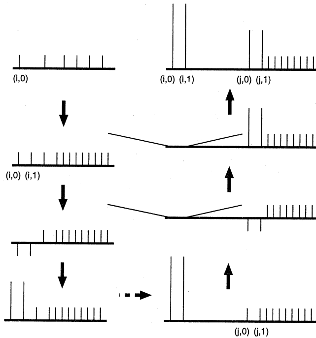
Figure 1: Algorithm
