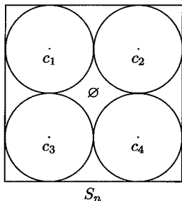
Figure 2: Perfect code illustration
