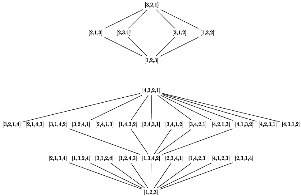
Figure 4: Hasse diagram for S_3 (top) and partial Hasse diagram for S_4 (bottom)
