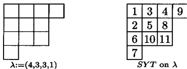
Figure 3: Young diagram and SYT
