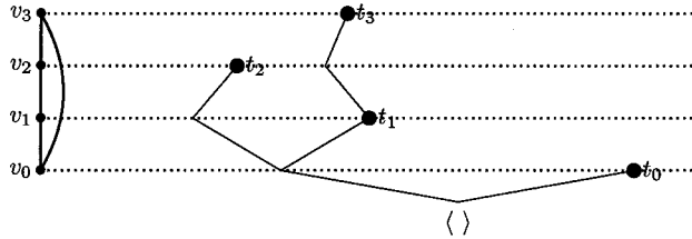
FIGURE 3. A tree coding a 4-cycle
