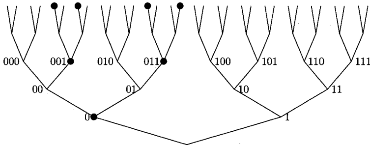
FIGURE 2. Another strong tree isomorphic to 2^{\leq 2}
