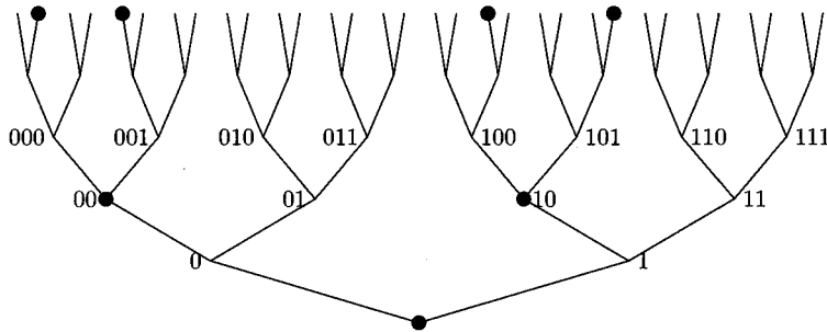
FIGURE 1. A strong tree isomorphic to 2^{\leq 2}
