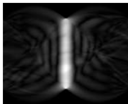
図 4: \alpha = \frac{1}{3}\pi , \mathcal{R}^{(\pi/3)} f
