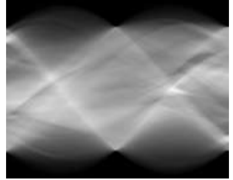
図 6: \alpha = \frac{1}{2}\pi , \mathcal{R}f
