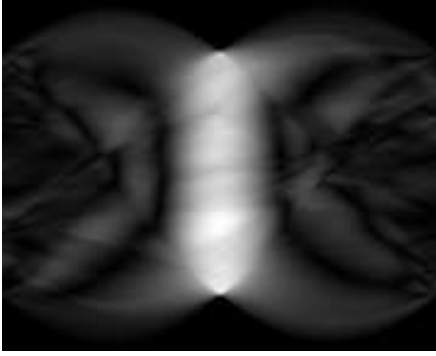
図 5: \alpha = \frac{5}{12}\pi , \mathcal{R}^{(5\pi/12)}
