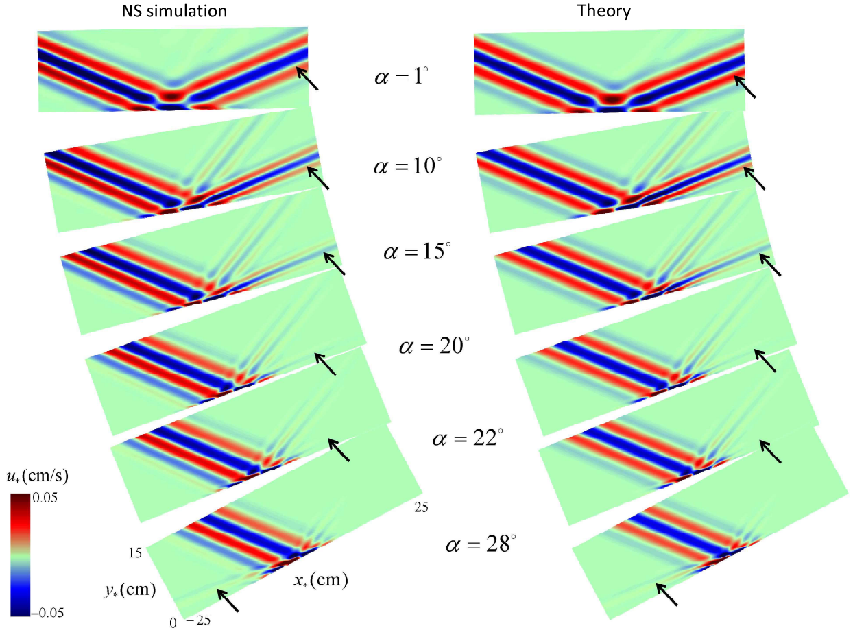
Figure 3 Comparison of NS simulation results (left column) and our theory (right column) for the x_* -velocity fields of beam reflection at fixed \theta = 22.7^\circ and Re = 100 . The incident beam profile is (16) with U_*^{\text{inc}} = 0.05\text{cm/s} , D_* = 3.5\text{cm} and L_* = 5\text{cm}/2\pi . From top, \alpha = 1^\circ, 10^\circ, 15^\circ, 20^\circ, 22^\circ , and 28^\circ . The primary-harmonic reflected beams are denoted by the black arrows.
