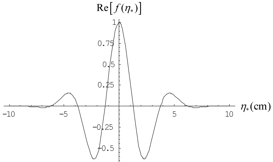
Figure 2. Profile of \text{Re}[f(\eta_*)] in (16) for D_* = 3\text{cm} and L_* = 5\text{cm} / 2\pi .
