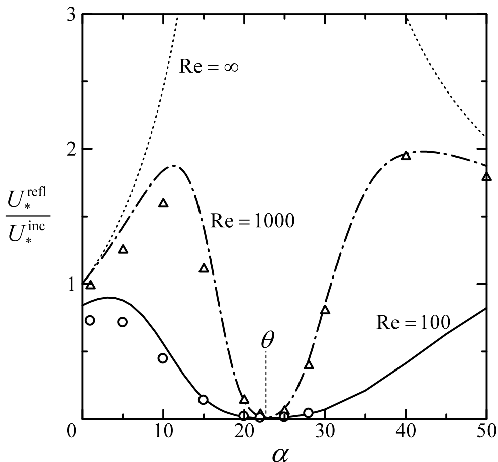
Figure 4 Ratio of reflected beam amplitude to incident beam amplitude U_*^{refl} / U_*^{inc} versus \alpha for \theta = 22.7^\circ . The solid, dash-dot, and dotted lines are the theoretical results for Re = 100, 1000 and \infty , respectively. The points are NS simulation results ( \circ : Re=100 , \triangle : Re=1000 ).
