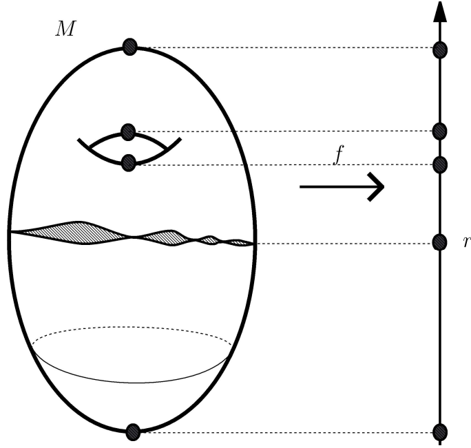
FIGURE 2. Non-triangulable function with finitely many critical values
