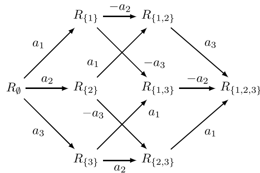
Figure 3: A 3-dimensional cube complex
