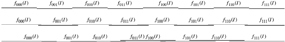
FIGURE 2. The intervals f_\omega(I) for \omega \in \{0, 1\}^3 when a = 0.5 (top), a = 0.52 (middle), and a = 0.58 (bottom).
