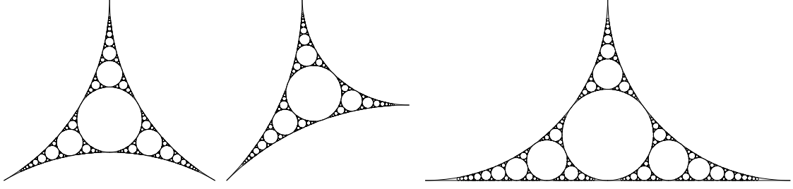
Figure 1: Apollonian gasket
