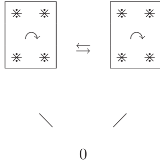
Fig. 3.13: Combinatorial multiradiality of \mathbb{F}_l^* -symmetries
