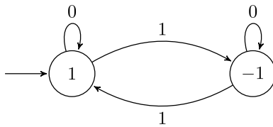
FIGURE 1. The 2-automaton producing the Thue–Morse sequence \{t(n)\}_{n \geq 0} .
