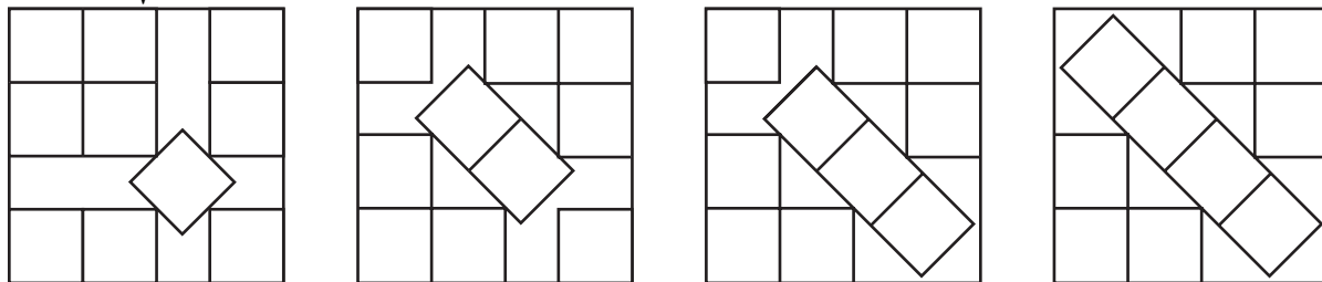
Figure 1: Best packings of 10 squares
