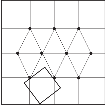
Figure 13: Ten points to avoid and how to avoid them
