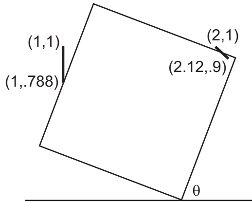
Figure 6: Proof of Lemma 5
