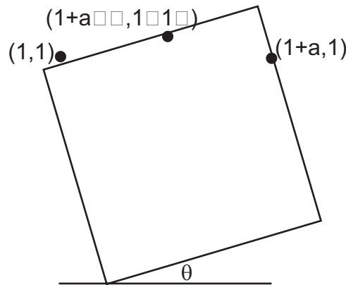
Figure 7: Proof of Lemma 6
