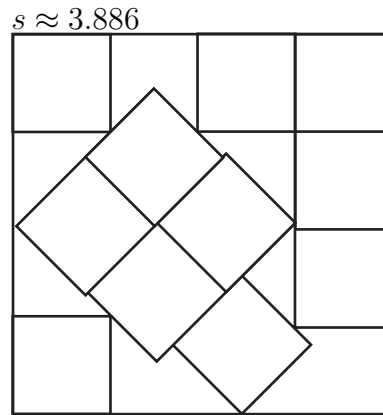
Figure 3: Optimal 45^\circ packing for n = 11
