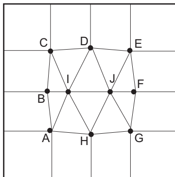
Figure 8: Each box contains one of these ten points
