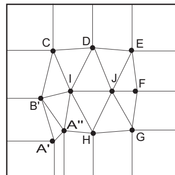
Figure 10: If A-box contains A'' , then H-box contains H'=(2,1)
