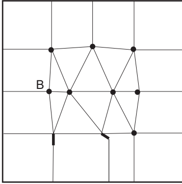
Figure 11: H-box must touch segment
