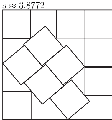
Figure 2: Best known packing of 11 squares (tilt \approx 40.182^\circ )
