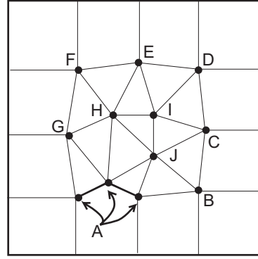
Figure 14: Twelve points for Theorem 2
