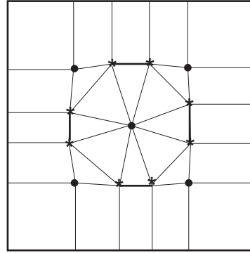
Figure 12: No room for I-box and J-box
