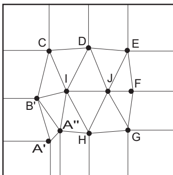
Figure 9: A-box contains one of A' , A''
