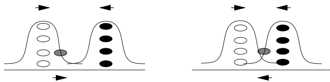
Figure 1: Two countermigrating ripple crests meet. The grey cell initially moves to the right (left plot), then reverses direction due to an encounter with (black) left moving cells. Later it will have a new encounter with (white) right moving cells (right plot).
