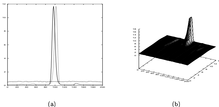
Figure 8: Formation of aggregates with \lambda as in (20). Parameters are a_* = 3 , \mu = 0.2 and p = 2 , 2800 steps are computed. Initial values and final shapes of the densities are given in (a). The evolution of the total density u = u^+ + u^- is shown in (b).
