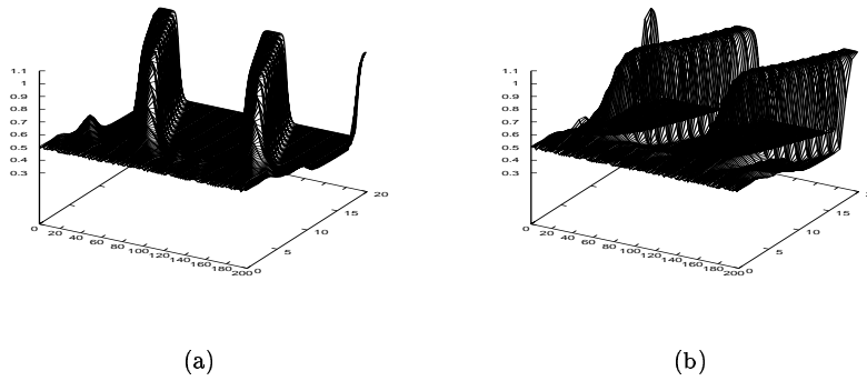
Figure 3: The evolution of ripples from a perturbation of the stationary state with \lambda as in (27). The densities u^+ (a) and u^- (b) are plotted every 4000 steps.
