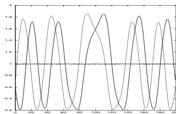
Figure 4: Initial and final density profiles of u^\pm with \lambda as in (28).
