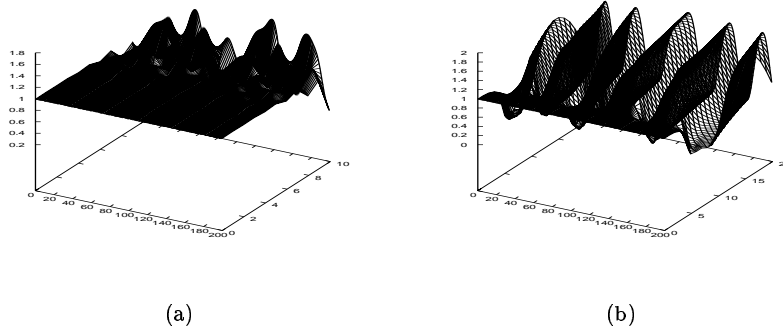
Figure 5: The evolution of ripples from a perturbation of the stationary state with \lambda as in (28). The profile of u^+ is plotted for the first 10 000 time steps (a) and for 40 000 steps (b). The ripples appear stationary because of the choice of time steps between each plot.
