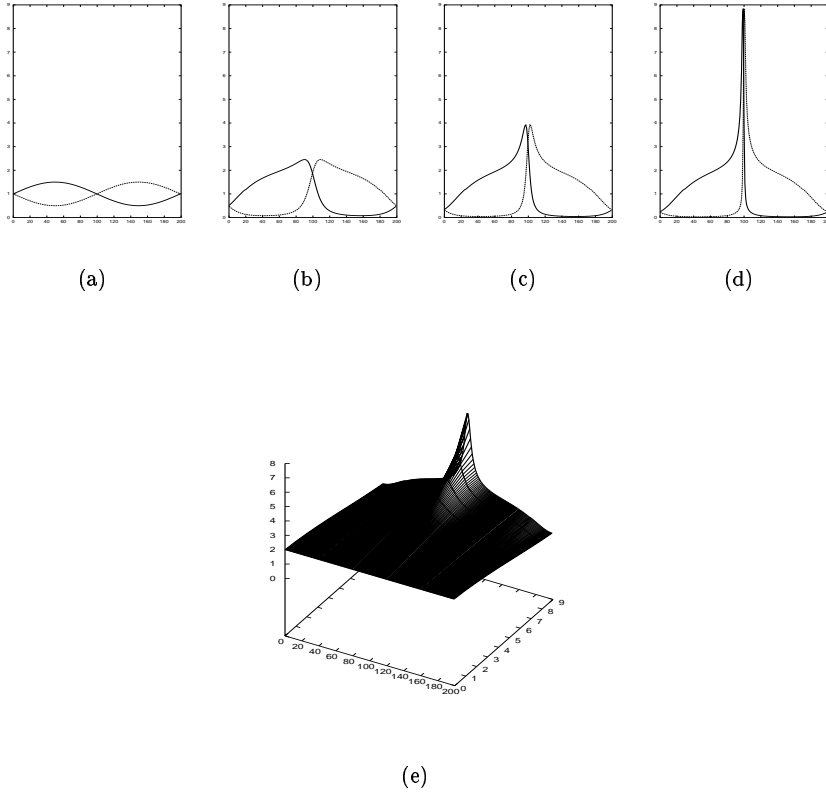
Figure 7: The profiles of u^\pm during the development of a peak with \lambda as in (47). An upwind scheme with 200 grid points is used. Parameters are a_* = 8, \mu = 0.1 . The plots are initial values (a), after 20 (b), 25 (c) and 30 (d) time steps. The time evolution of the total density u = u^+ + u^- is given in (e).
