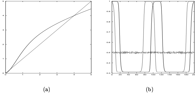
Figure 2: The shape of f from (27) and the shapes of the two densities u^\pm at the beginning and the end of the simulation.
