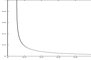
Figure 6: The wavelength l of ripples as a function of the fraction of C-signaling capable cells \beta given in (41) with a = c = 1, \mu = 10^{-2}, \varepsilon\pi^2 = 10^{-3} .
