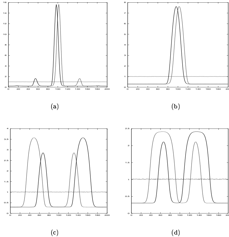
Figure 9: Emerging patterns with \lambda as in (20) for increasing q and increasing time interval. Parameters are a_* = 3, b_* = 1, \mu = 0.2 and p = 2 . (a) has q = 1.2 and 4000 time steps, (b) has q = 1.5 and 24 000 time steps, (c) has q = 2.2 and 40 000 time steps and (d) has q = 2.5 and also 40 000 time steps. Note the different scales on the vertical axis. Whereas the maximum in (a) is almost 16 and in (b) almost 8, it is only about 3.5 in (c) and merely 2.5 in (d).
