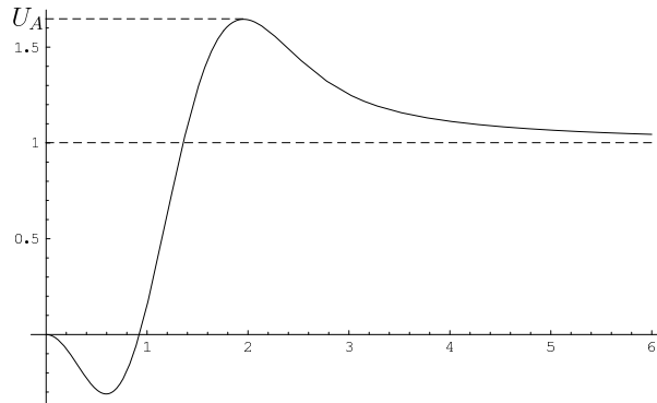
Figure A.1: Graph of U(z) on the positive real axis. (The same figure as [BB, Fig.3, in p.656].)
