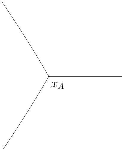
Figure A.2: Stokes curves near x_A (i.e., in the region \{x; |\operatorname{Re}(x - x_A)| < 0.2, |\operatorname{Im}(x - x_A)| < 0.2\} ).
