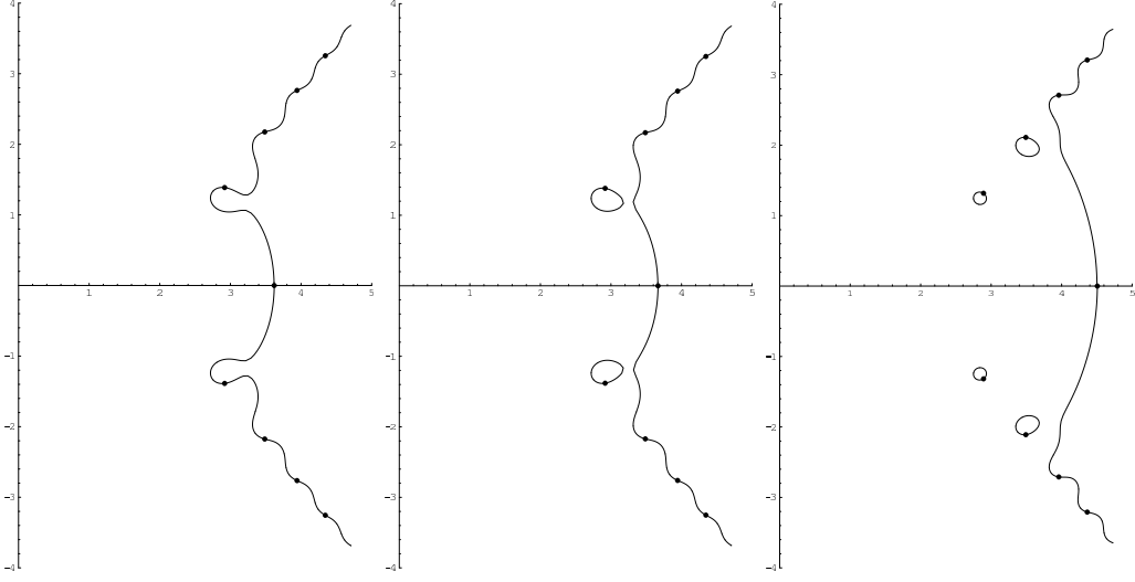
Figure A.4: Locus of z(x) with different r 's ( r = 0.066 (left), r = 0.064 (middle) and r = 0.040 (right)).
